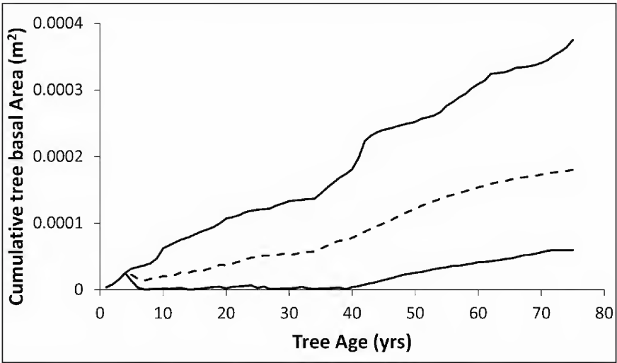
FIGURE 5. Cumulative basal area ( \text{m}^2 ) for an average Picea mariana tree in the six plots. Solid lines indicate the maximum and minimum cumulative basal area for trees at a given age; the dashed line represents the average ( n = 156 ). The shallow slope of the average basal area growth curve suggests that growth was extremely slow throughout the life of a given tree in the stand.
